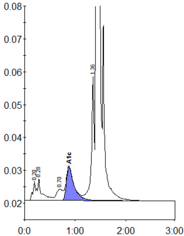
Peak table - ID: 10443626
